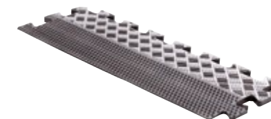
LMX1351 Rubber floor edge Made of high density rubber | Dimensions: L: 500mm x W: 160mm x H: 10mm | Sloping | Colour: black
