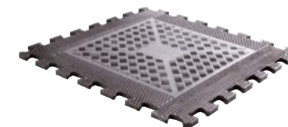
LMX1350 Rubber floor mat Made of high density rubber | Dimensions: L: 500mm x W: 500mm x H: 10mm | Colour: black
